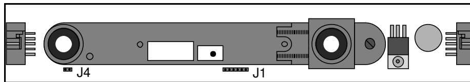
Configuration 1 - SMR: Jumper: J1 “6 Pin” and J4 (Earliest Slave Module)
