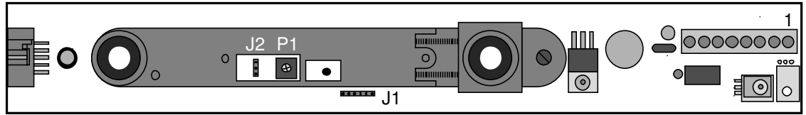
Configuration 3 – Non SMR: Jumpers: J1 “6 Pin” and J2 (Latest Master Module)
