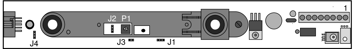
Configuration 2 - SMR: Jumpers: J1 “3 Pin”, J2, J3 and J4 (Subsequent Master Module)
