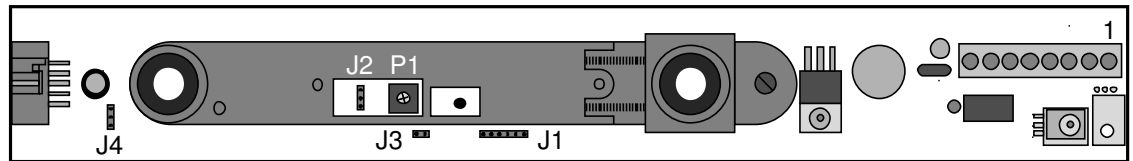
Configuration 1 - SMR: Jumpers: J1 “6 Pin”, J2, J3 and J4 (Earliest Master Module)
