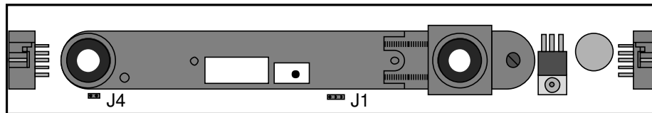
Configuration 2 - SMR: Jumper: J1 “3 Pin” and J4 (Subsequent Slave Module)
