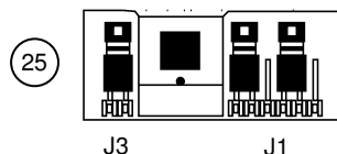
6-Pin Normal Mode (Default)
