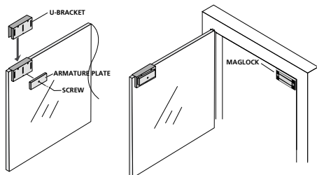
U-Bracket and Glass Door
