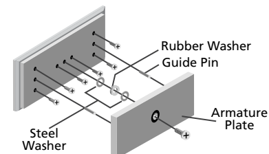
Armature Plate Assembly
