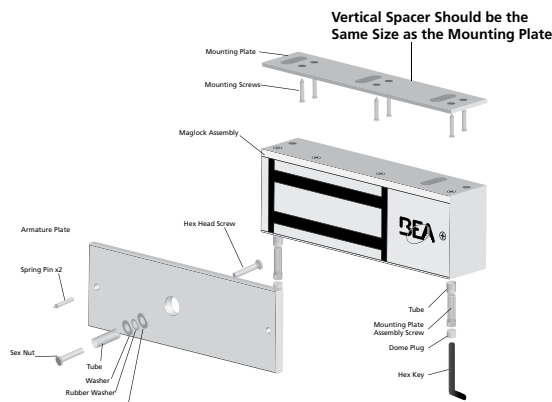
Vertical Spacer and Armature Plate
