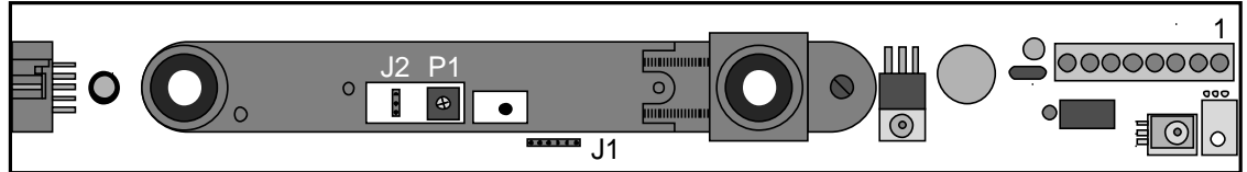
Configuration 3 – Non SMR: Jumpers: J1 “6 Pin” and J2 (Latest Master Module)
